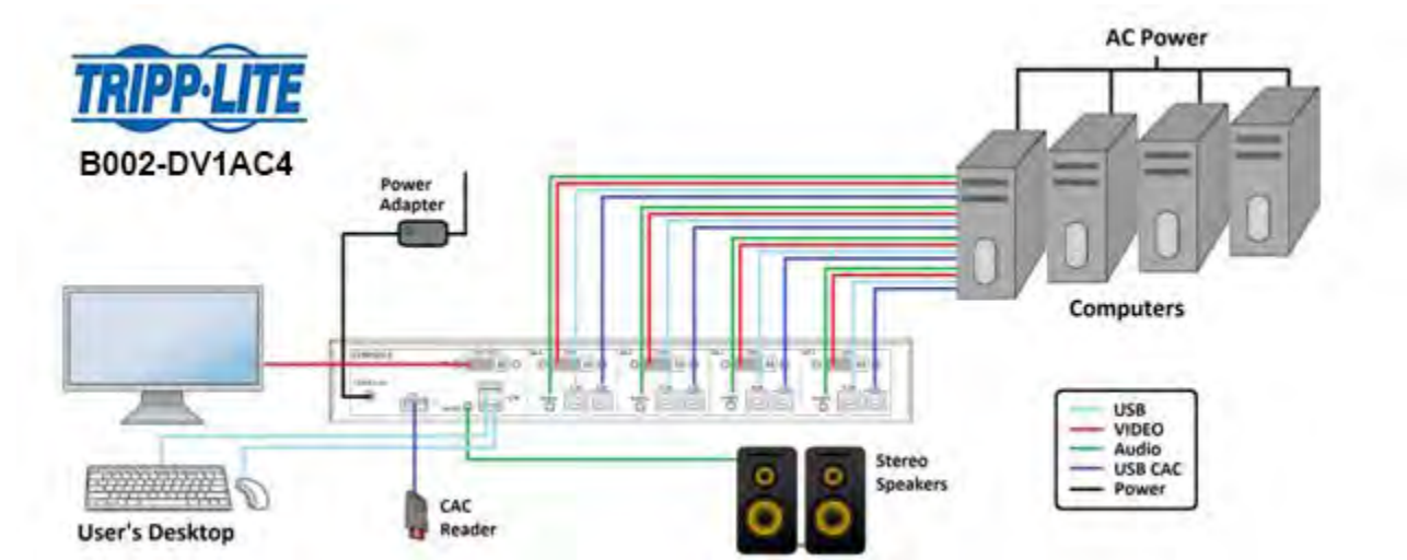
Figure 1: Standard Setup of 4-Port KVM TOE Installation
