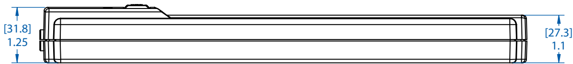
SIDE VIEW
