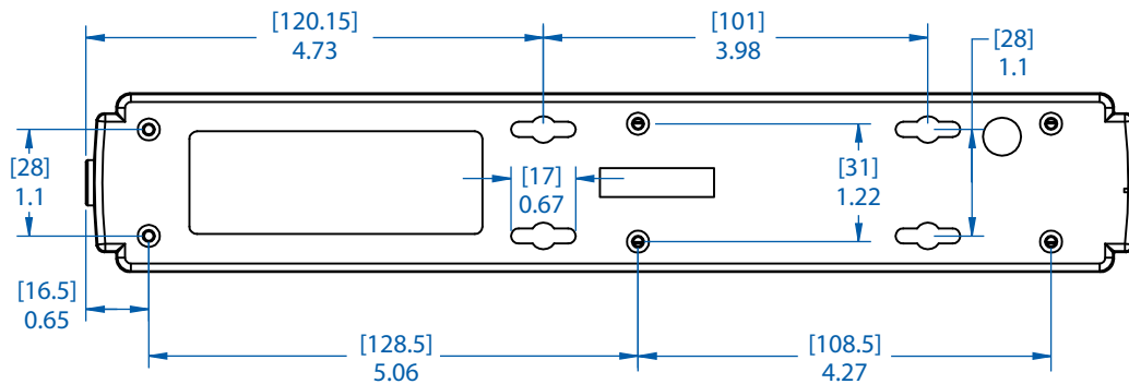
BOTTOM VIEW
