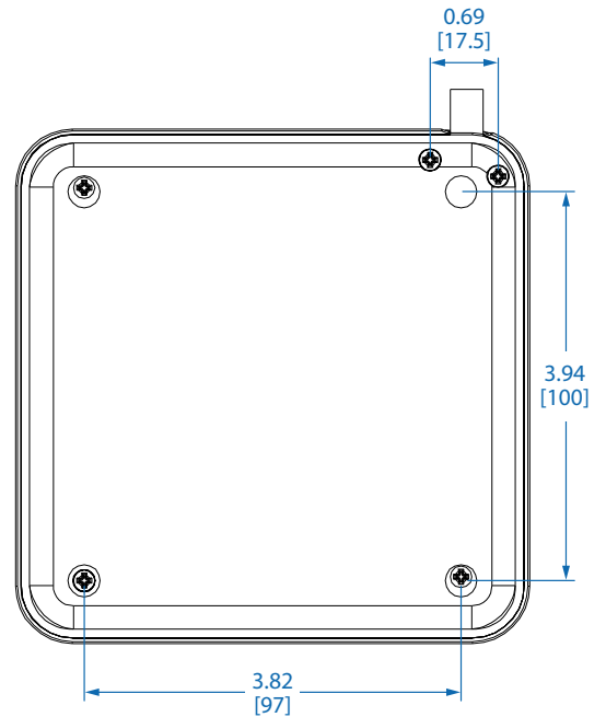
BOTTOM VIEW
