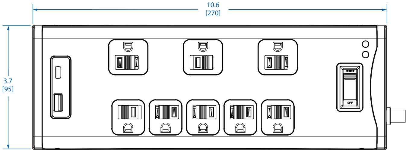
TOP VIEW
