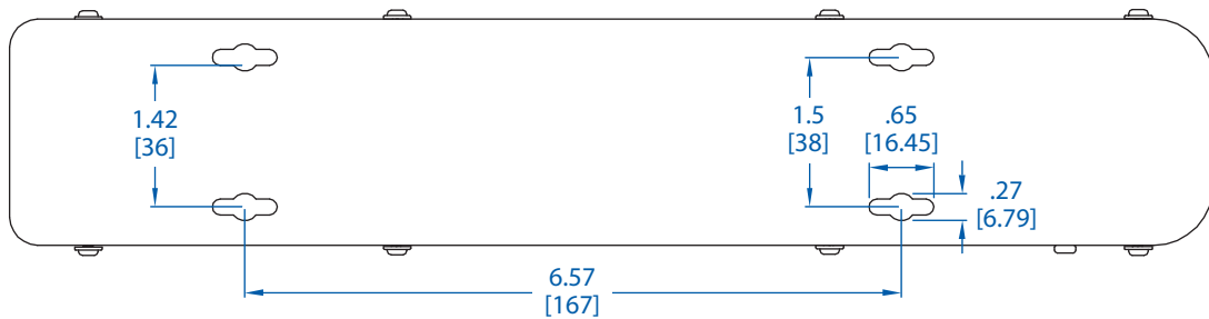
BOTTOM VIEW
