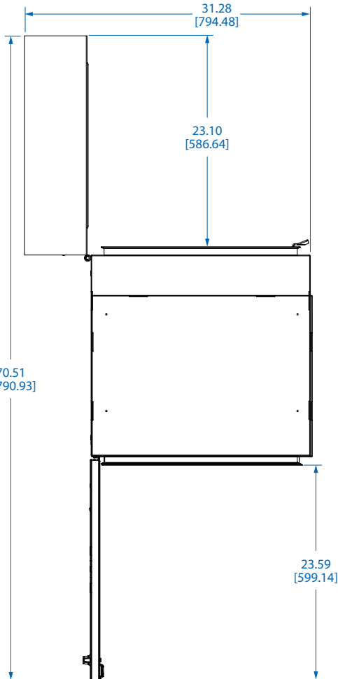
TOP VIEW WITH DOOR OPEN
