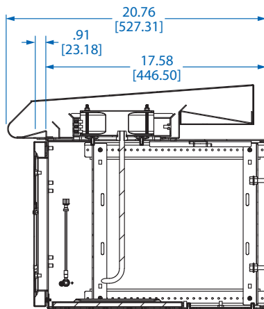
SECTION A
