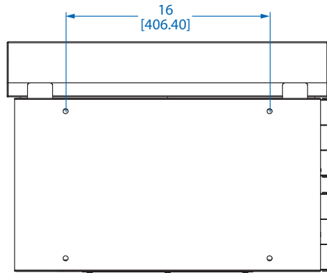
BACK VIEW
