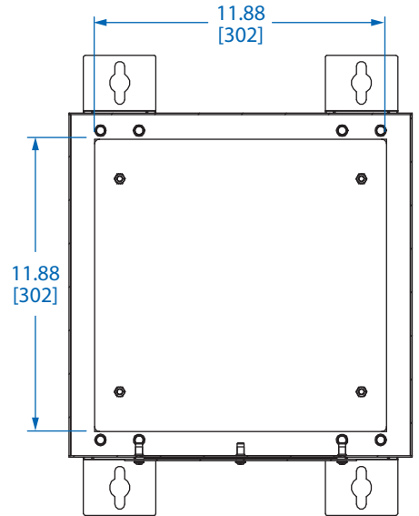
BACK VIEW
