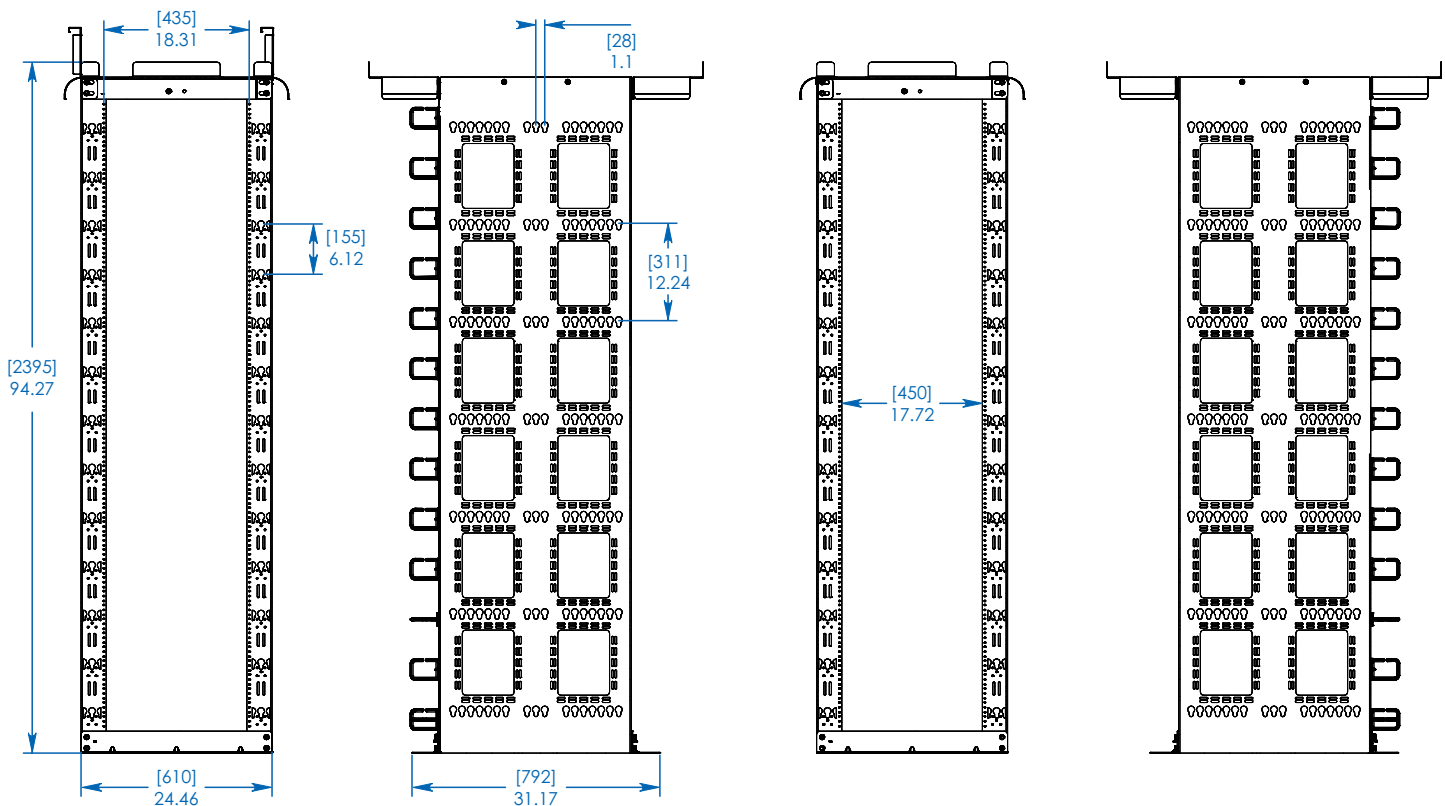
FRONT
