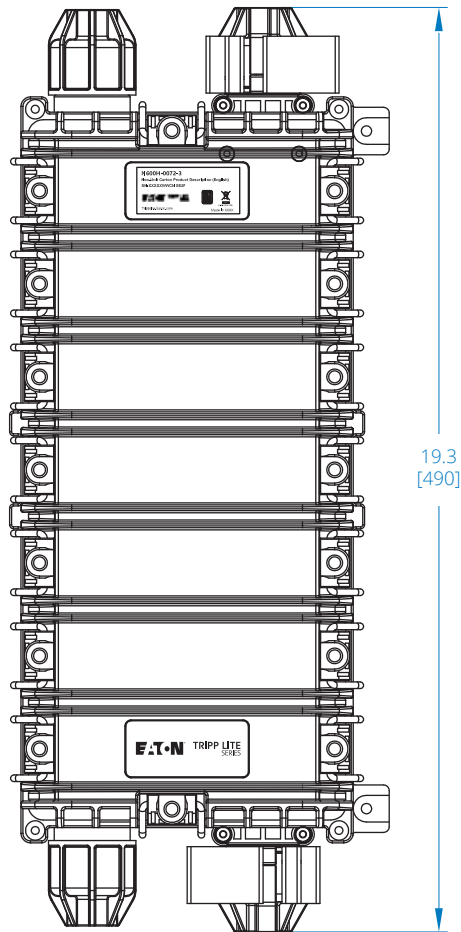
FRONT VIEW
