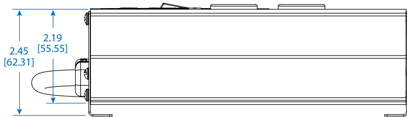
SIDE VIEW
