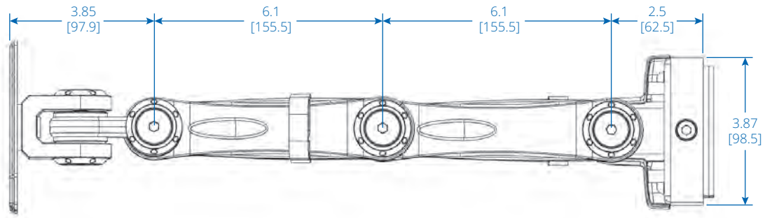
TOP VIEW
