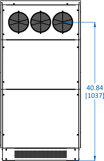
Rear view
