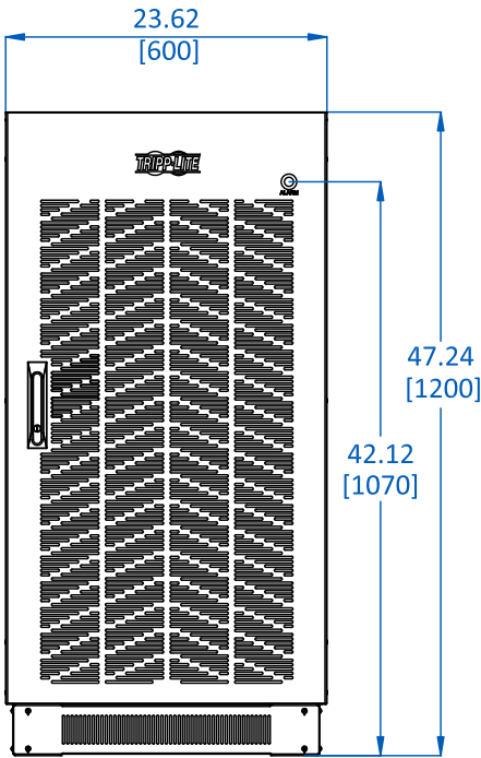
Front view
