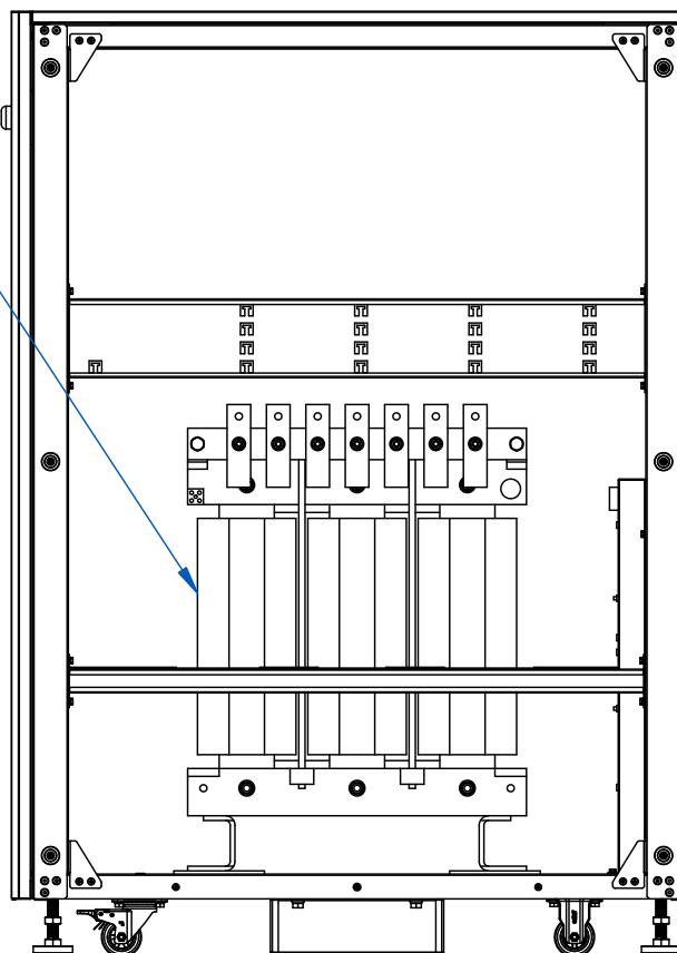
Side view (remove cover)
