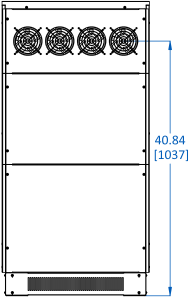
Rear view
