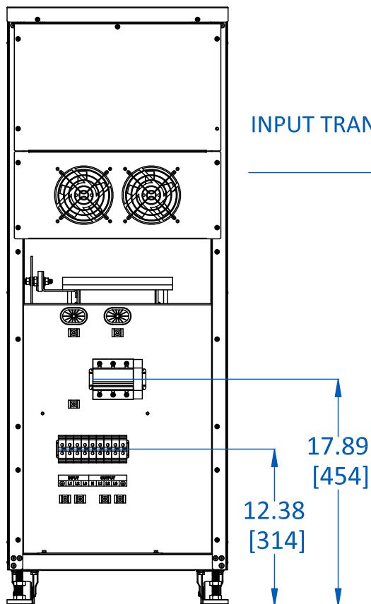
Rear view (remove cover)
