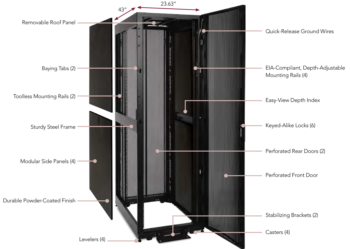
42U Standard-Width, Standard-Depth Cabinet with Side Panels
